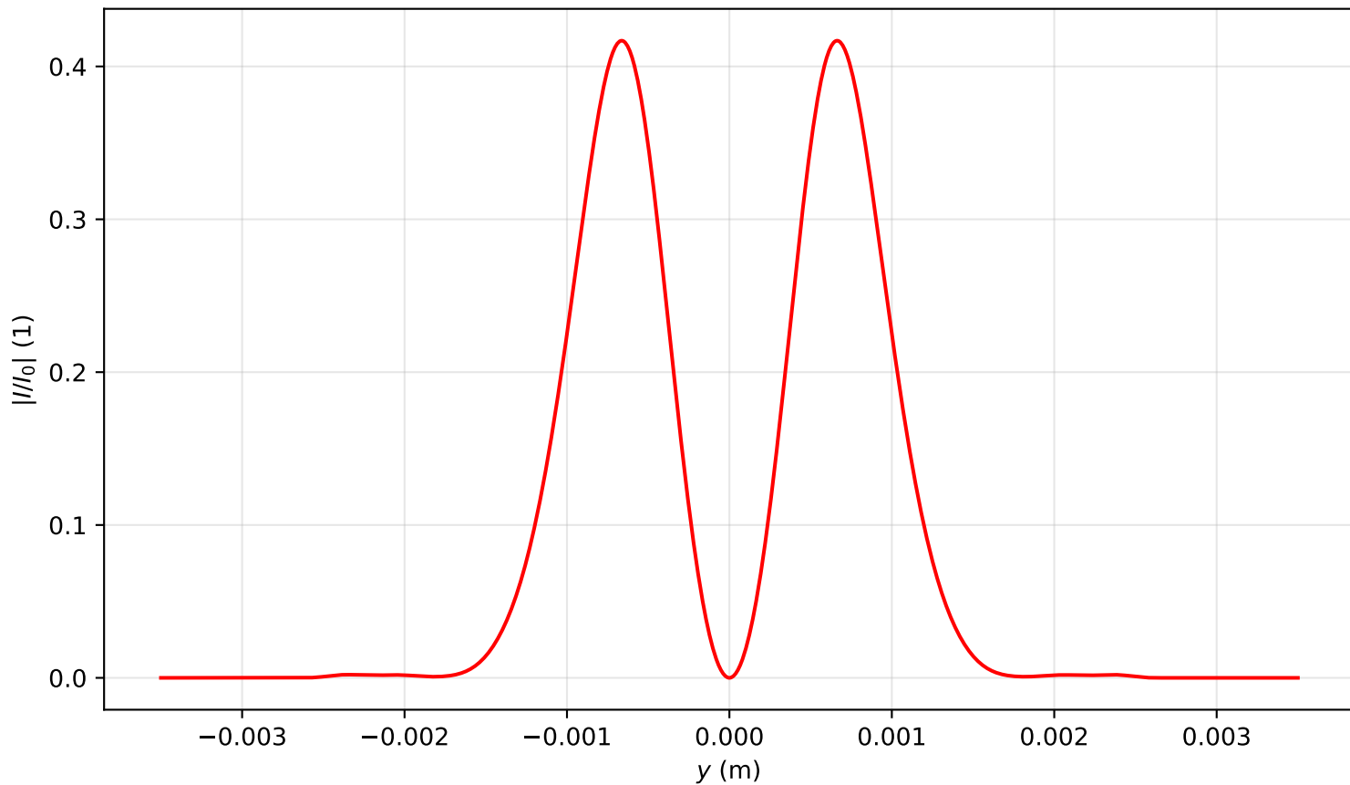
Intensity profile I(x=0, y, z=2.149)/I_0 , \text{Pin}=3.0\text{Pcr} , artificial time
